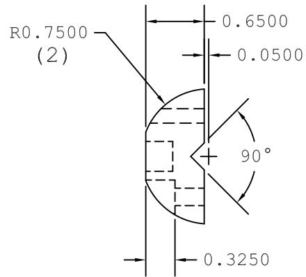
CLAMP 2 PCS
