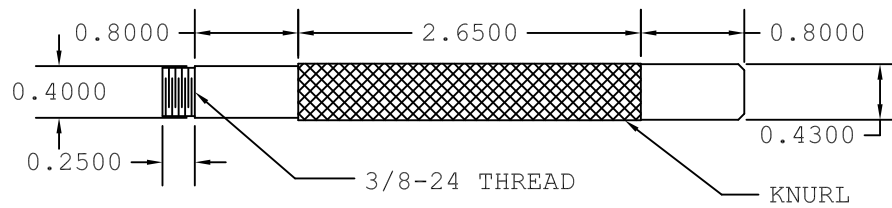
HANDLE (2 PCS) 7/16" X 4.5" ROUND ROD
