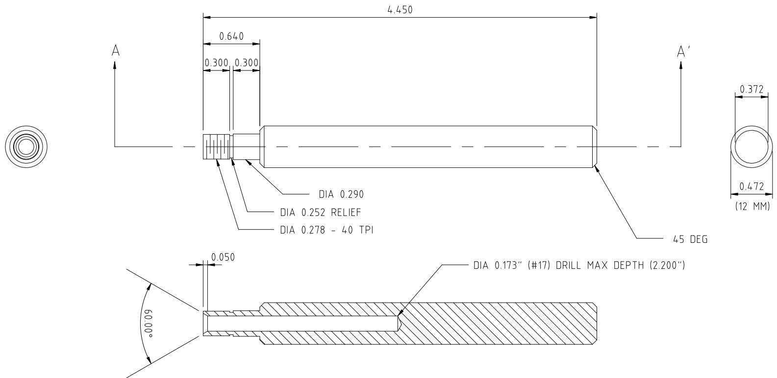
CROSS-SECTION A-A'
