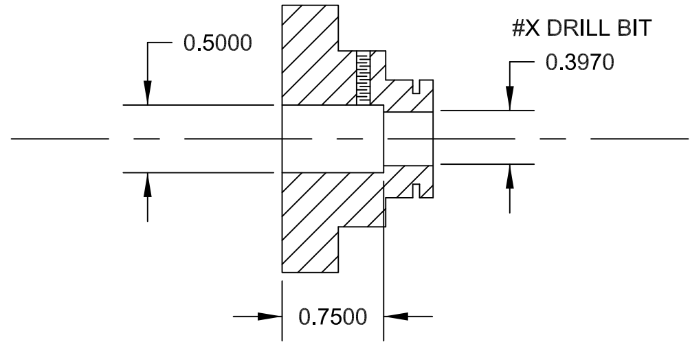
DIAL KNOB CROSS SECTION
