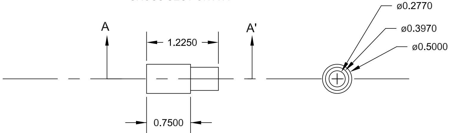
DIAL KNOB INSERT
