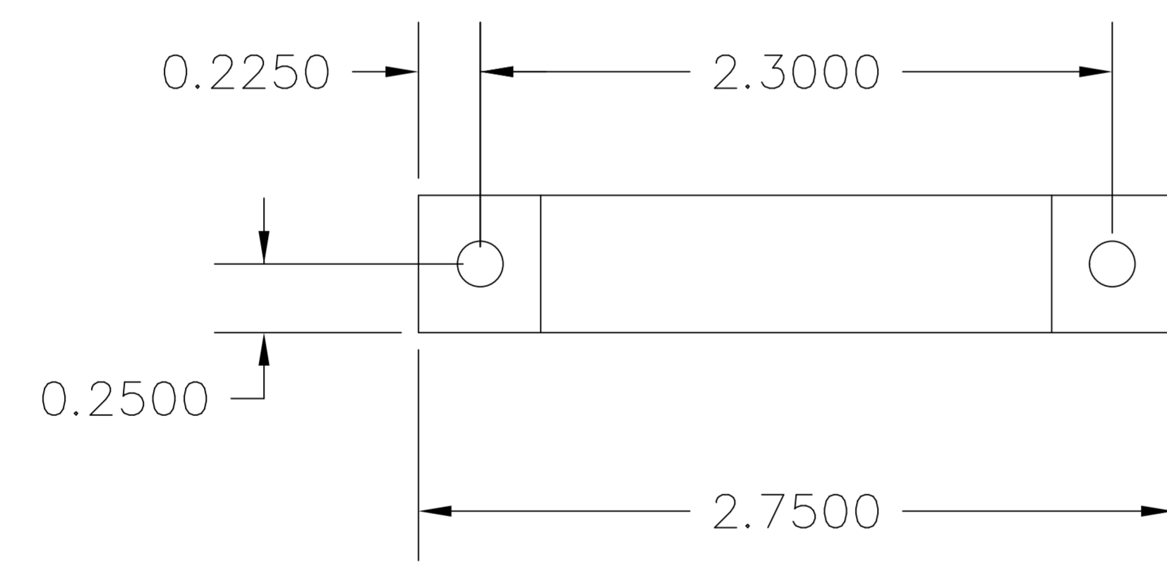
CLAMP
